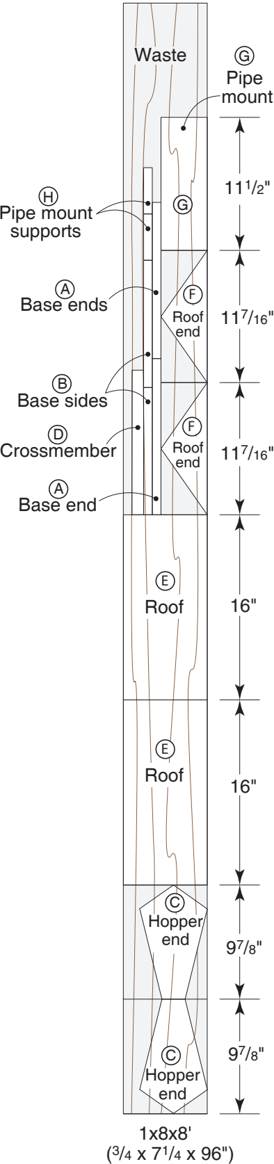
CUTTING DIAGRAM
