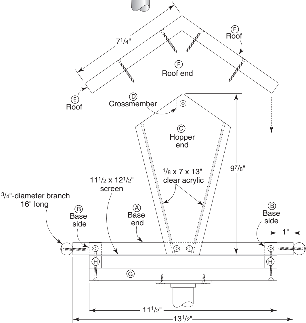
END VIEW
