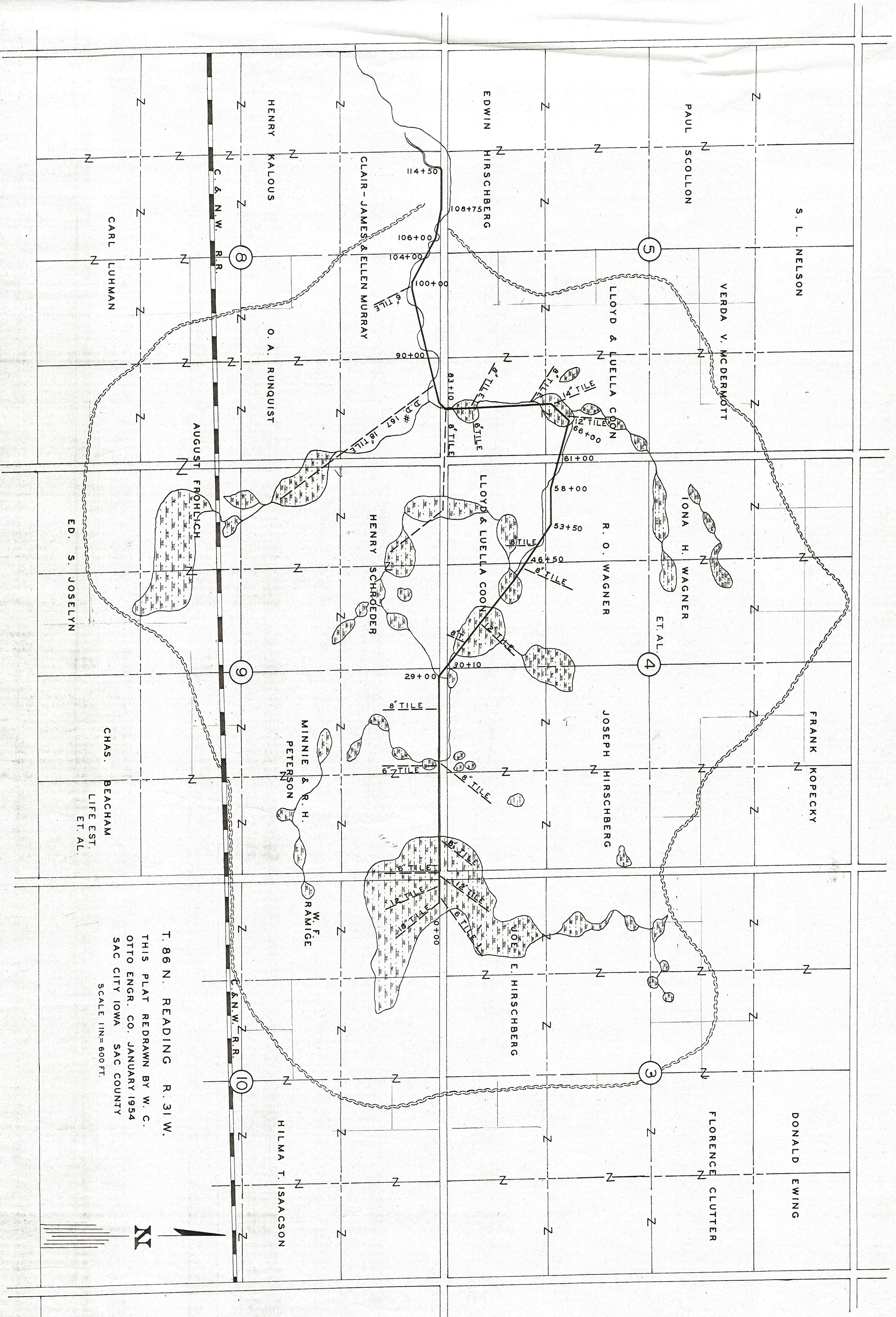
PLAT OF DRAINAGE DISTRICT No. 18 LOCATED ON SEC. 3-4-5-8-9-10 T. 86 N. R. 31 W. OF 5 TH P.M.
